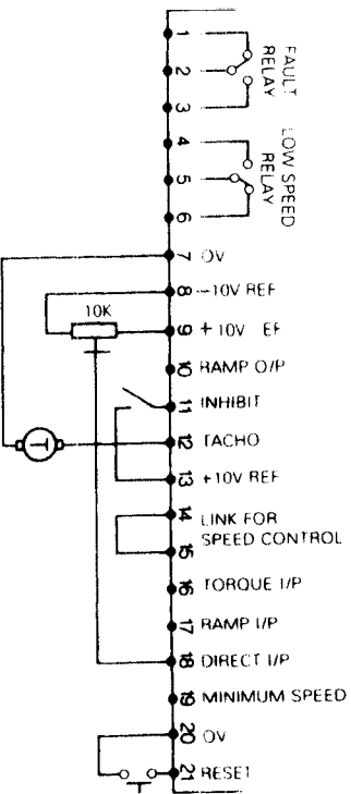
CONTROL TERMINAL CONNECTIONS
