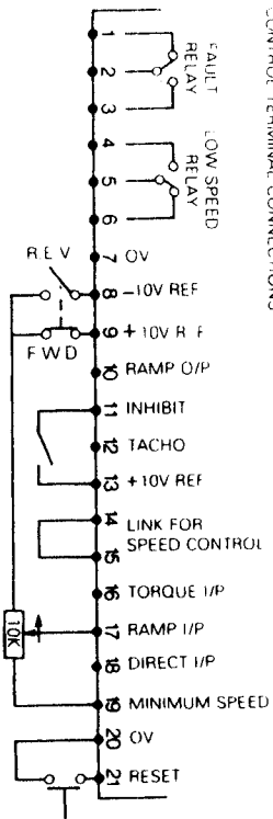
CONTROL TERMINAL CONNECTIONS
